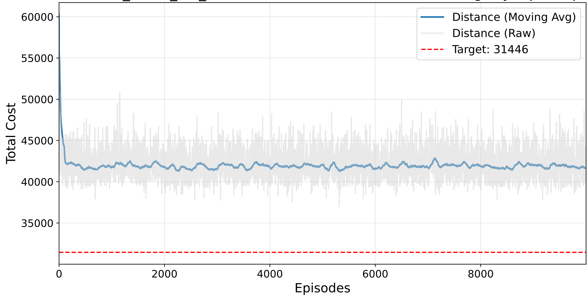
Final NO_MASK_NO_BAYESIAN Masked AutoRL-SOP Training - ry48p.4.sop
